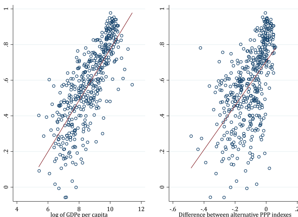
Figure 2, Correlation between expenditure shares of each country and the US across benchmark comparisons compared with income levels and PPP precision
